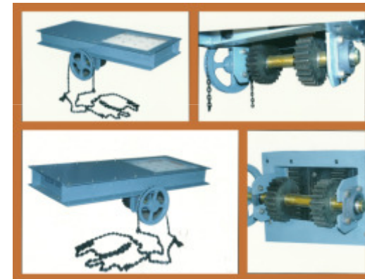
Slide Gate for Ash Hopper
